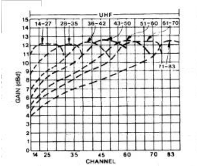
J-275D - ** GAIN CURVES
